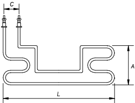
MANIFOLD HEATER
