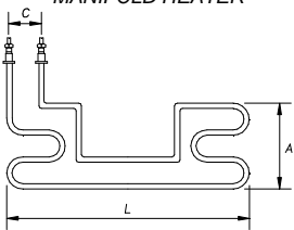
MANIFOLD HEATER
